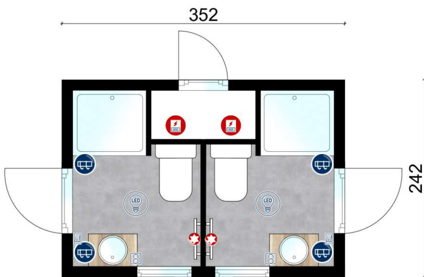
Eos KUN-MBH-002423 3,52 x 2,42 m
